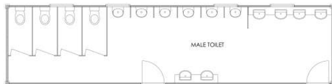
MALE TOILET MODULE (40FMOMTOIL01) 12192 OR 6096 x 3000 x 2896 at 2500kg - 6000kg approx
