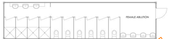
FEMALE ABLUTION MODULE (40FMOFABLU01) 12192 OR 6096 x 3000 x 2896 at 2500kg - 6000kg approx
